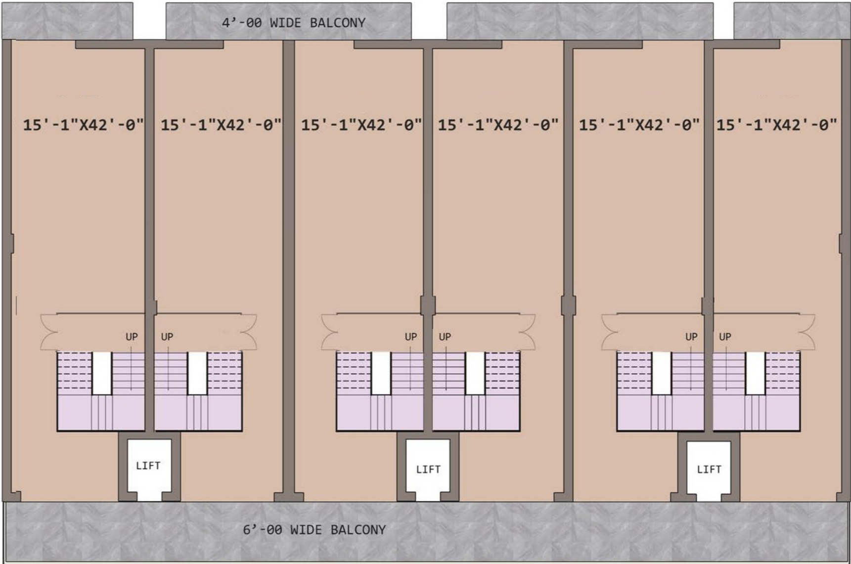
SECOND & THIRD FLOOR PLAN
